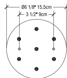
CANOPY - BOTTOM VIEW
