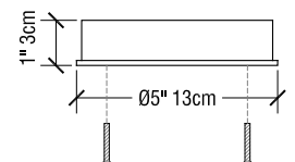
CANOPY - SIDE VIEW
