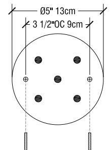
CANOPY - BOTTOM VIEW
