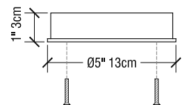
CANOPY - SIDE VIEW
