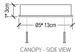
CANOPY - SIDE VIEW
