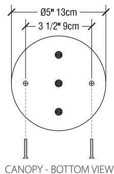
CANOPY - BOTTOM VIEW
