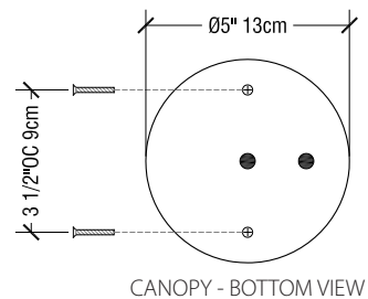
CANOPY - BOTTOM VIEW
