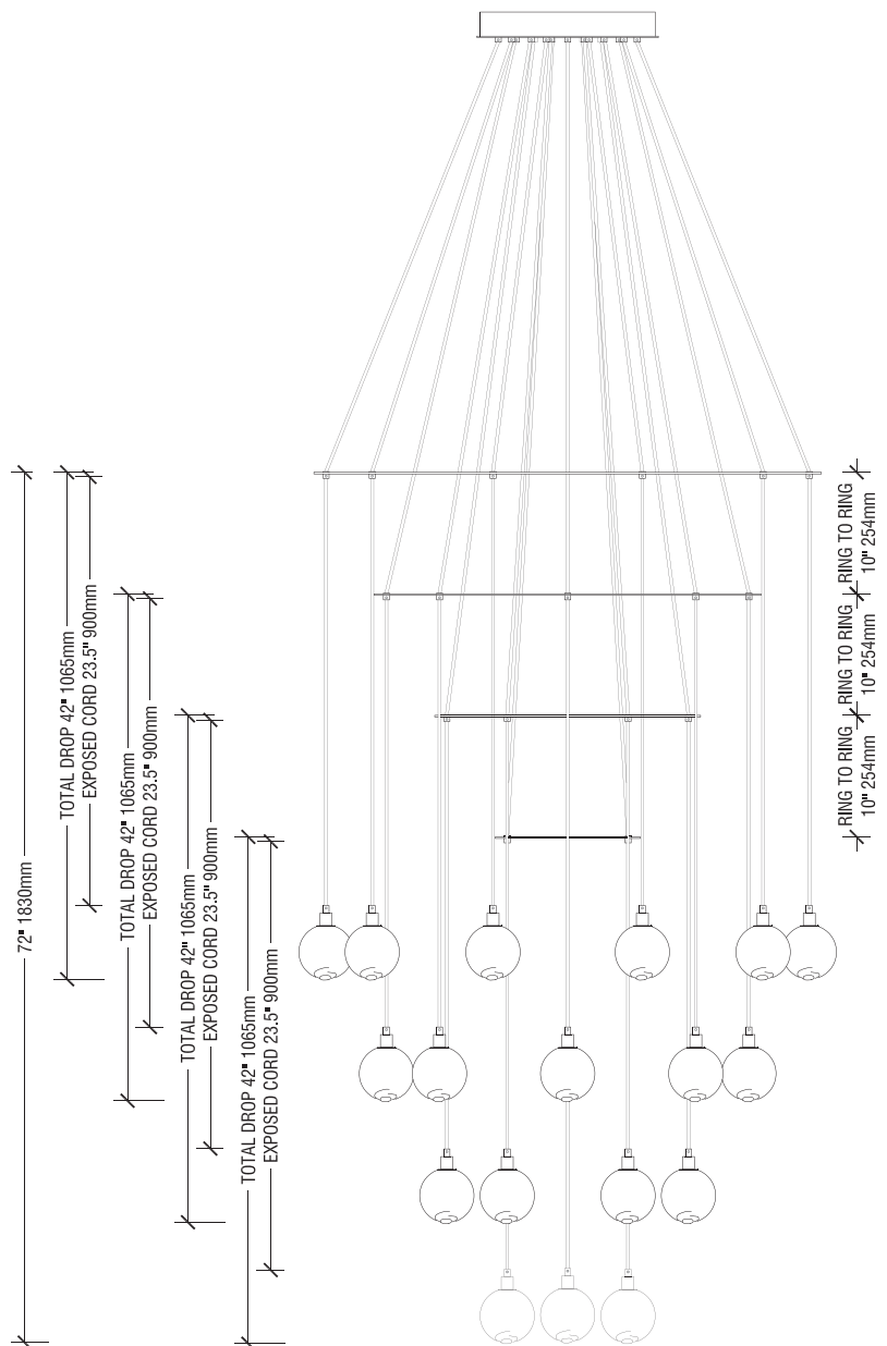
Figure 5. Standard fixture composition dimensions
