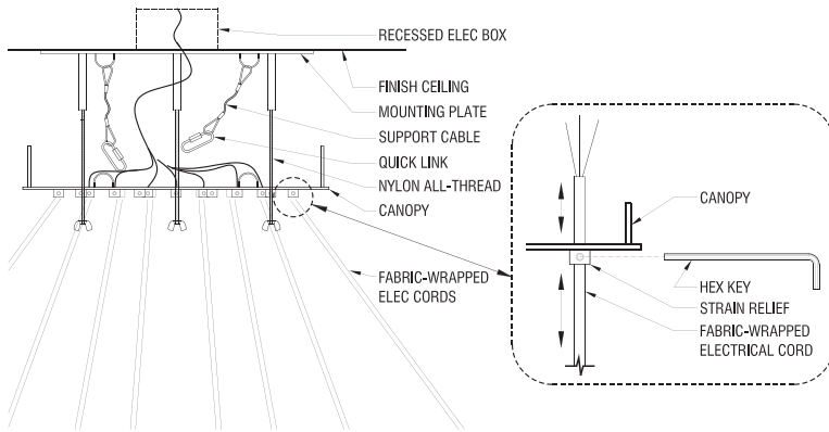
Figure 6. Leveling the fixture
