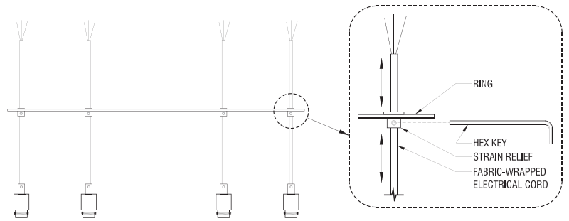
Figure 4. Pass cords through rings
