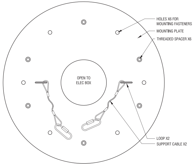
Figure 2. Install mounting plate
