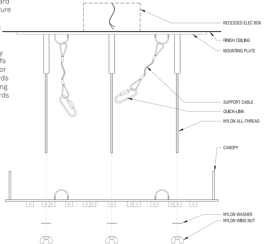
Figure 3. Install nylon all-thread rods into mounting plate and slide canopy up over rods
