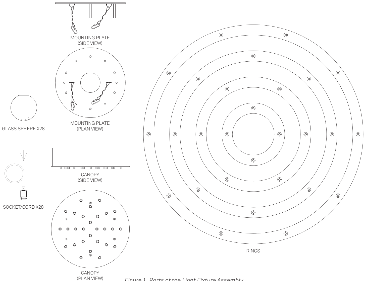
Figure 1. Parts of the Light Fixture Assembly
