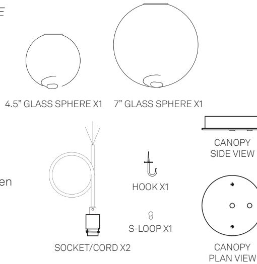
Figure 1. Parts of the Light Fixture Assembly
