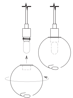
Figure 4. Install glass spheres by threading onto brass sockets
