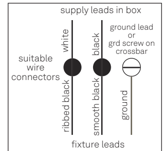
Figure 2. Wiring Diagram
